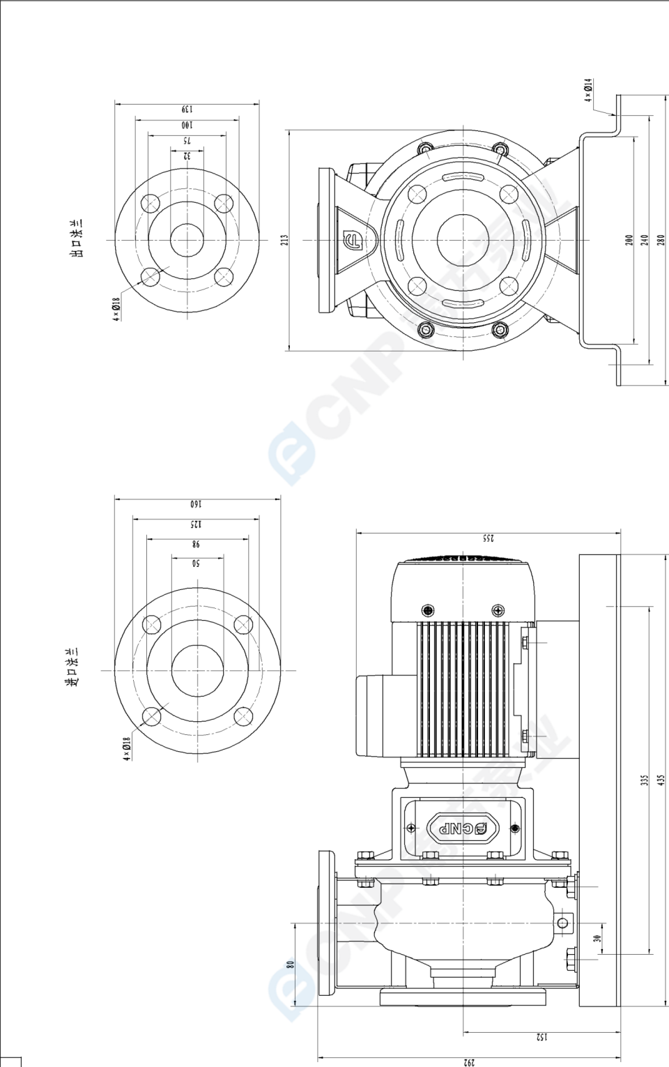
ZM50-32-125T/0.55
