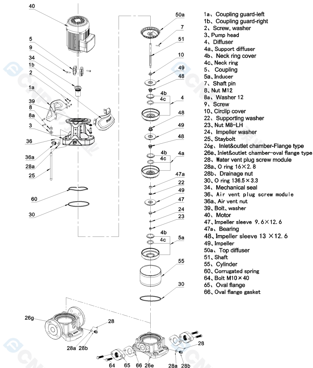
Drawing 1-D CDM5-240703
